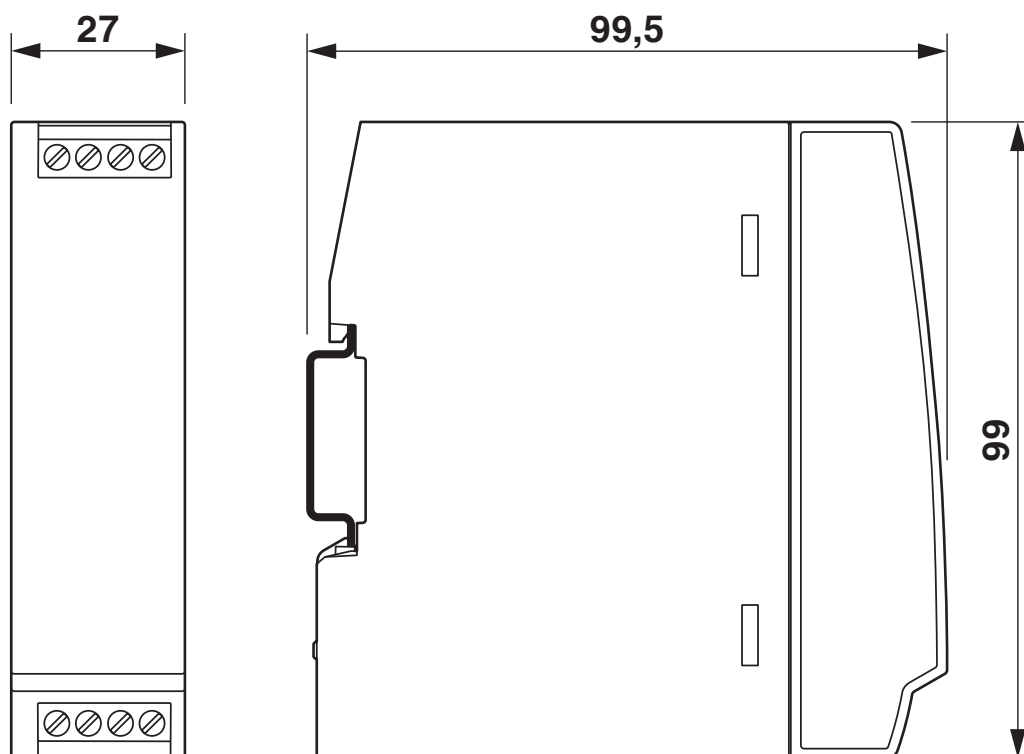
Dimensional drawing
