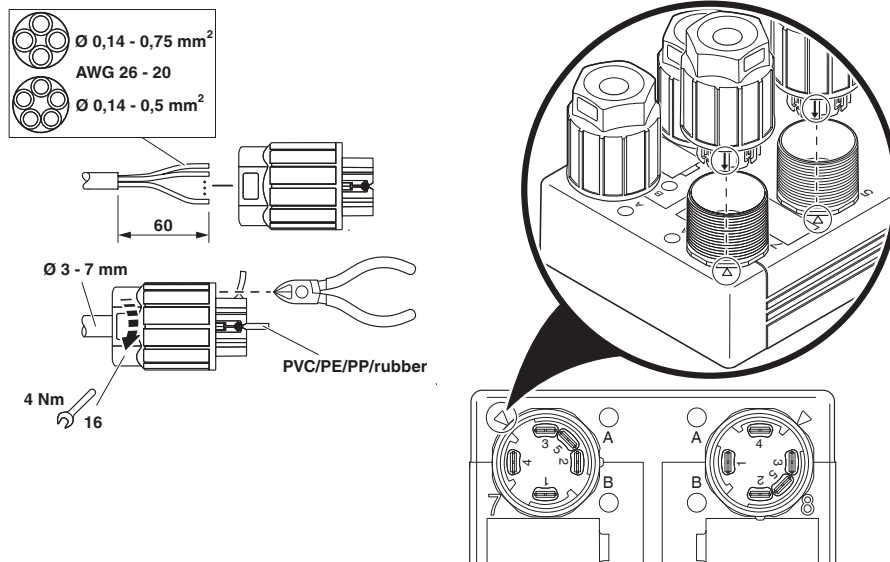
Functional drawing
