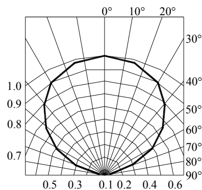
Fig.6 Relative Intensity vs. Angle
