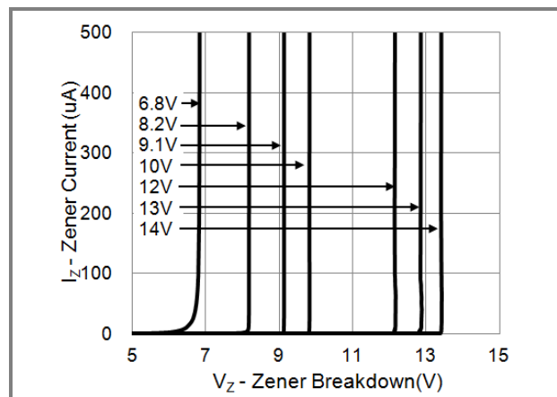
Fig.4 Typical Zener Breakdown
