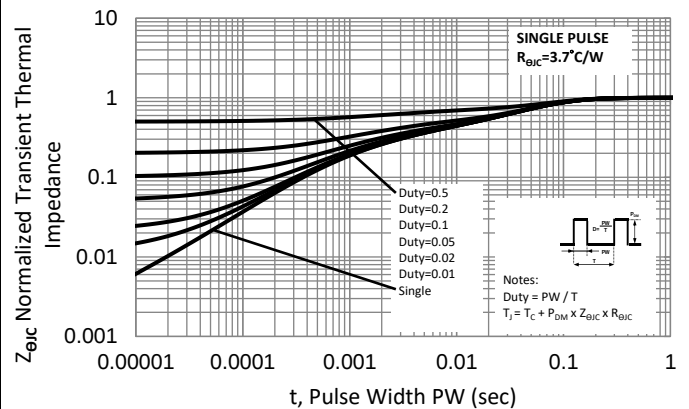
Fig.12 Normalized Transient Thermal Impedance
