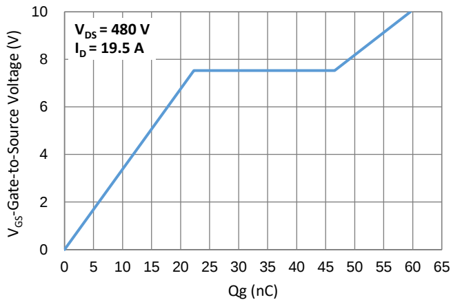
Fig.7 Gate-Charge Characteristics
