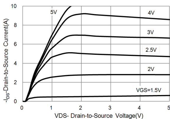
Fig.1 On-Region Characteristics
