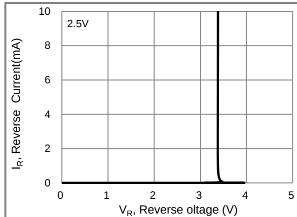
Fig.10 Typical Reverse Characteristics
