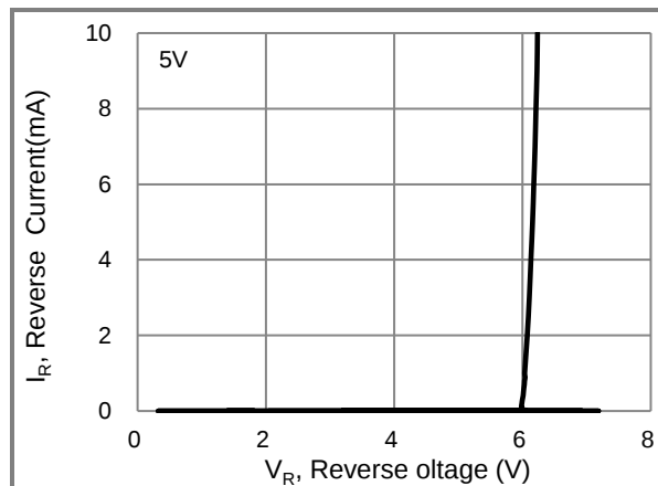
Fig.12 Typical Reverse Characteristics
