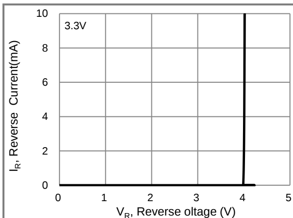
Fig.11 Typical Reverse Characteristics
