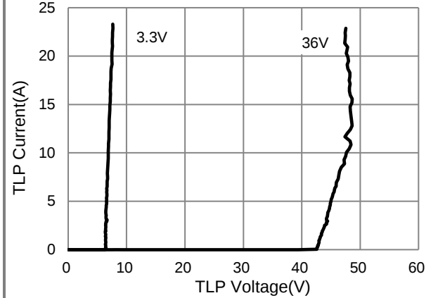
Fig.2 TLP Measurement
