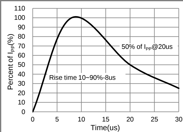
Fig.3 Pulse Waveform
