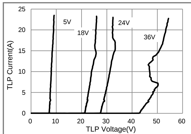
Fig.6 TLP Measurement
