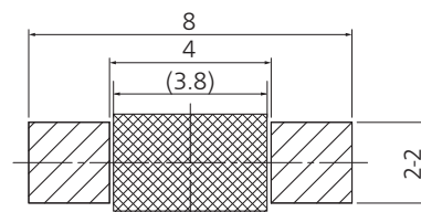
PWB land pattern for reference
