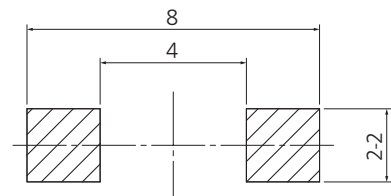
PWB land pattern for reference
