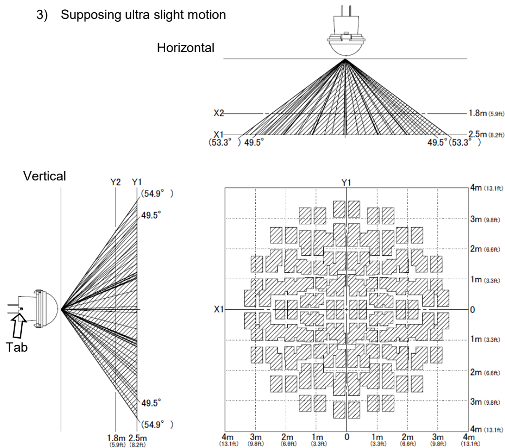
X-Y Cross Section (2.5m) (8.2ft)
