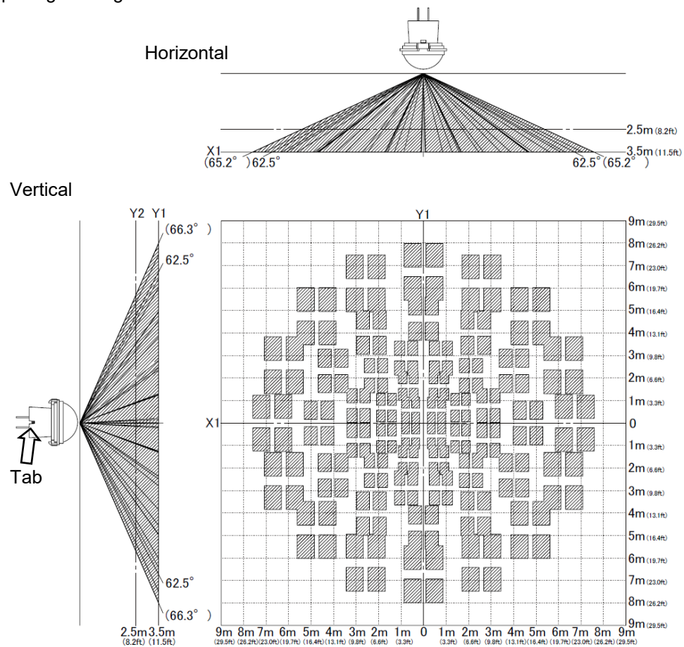
X-Y Cross Section (3.5m) (11.5ft)
