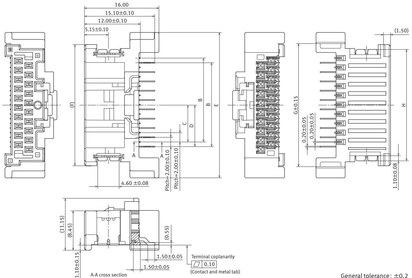
External dimensions
