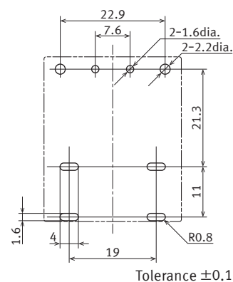
Schematic ( BOTTOM VIEW )
