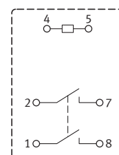
Schematic ( BOTTOM VIEW )
