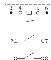
Schematic ( BOTTOM VIEW )
