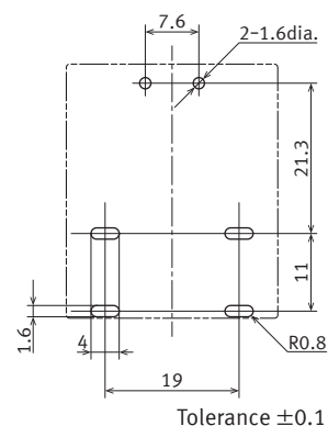
Recommended PC board pattern ( BOTTOM VIEW )
