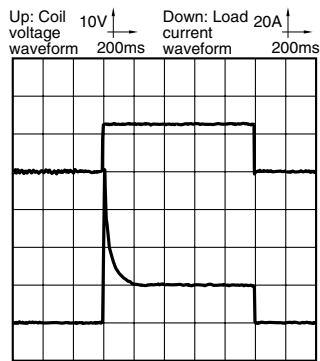
Load current waveform Inrush current: 90A, steady current: 20A
