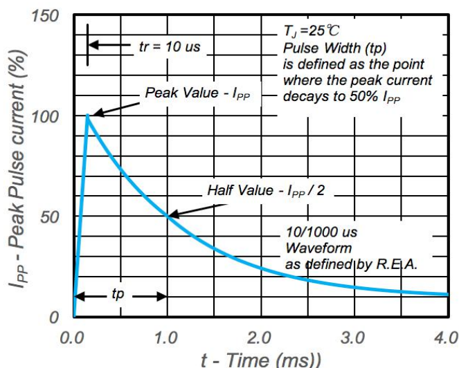
Fig.3 Pulse Waveform
