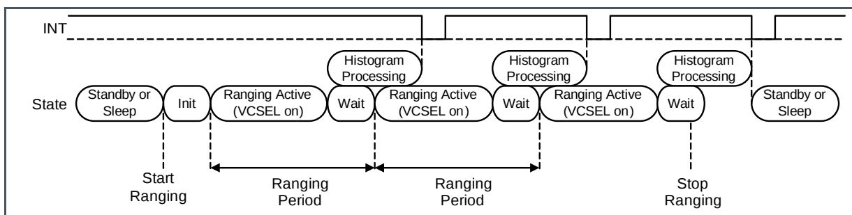
Figure 26: Timing Diagram for Ranging Period < Ranging Active + Histogram Processing
