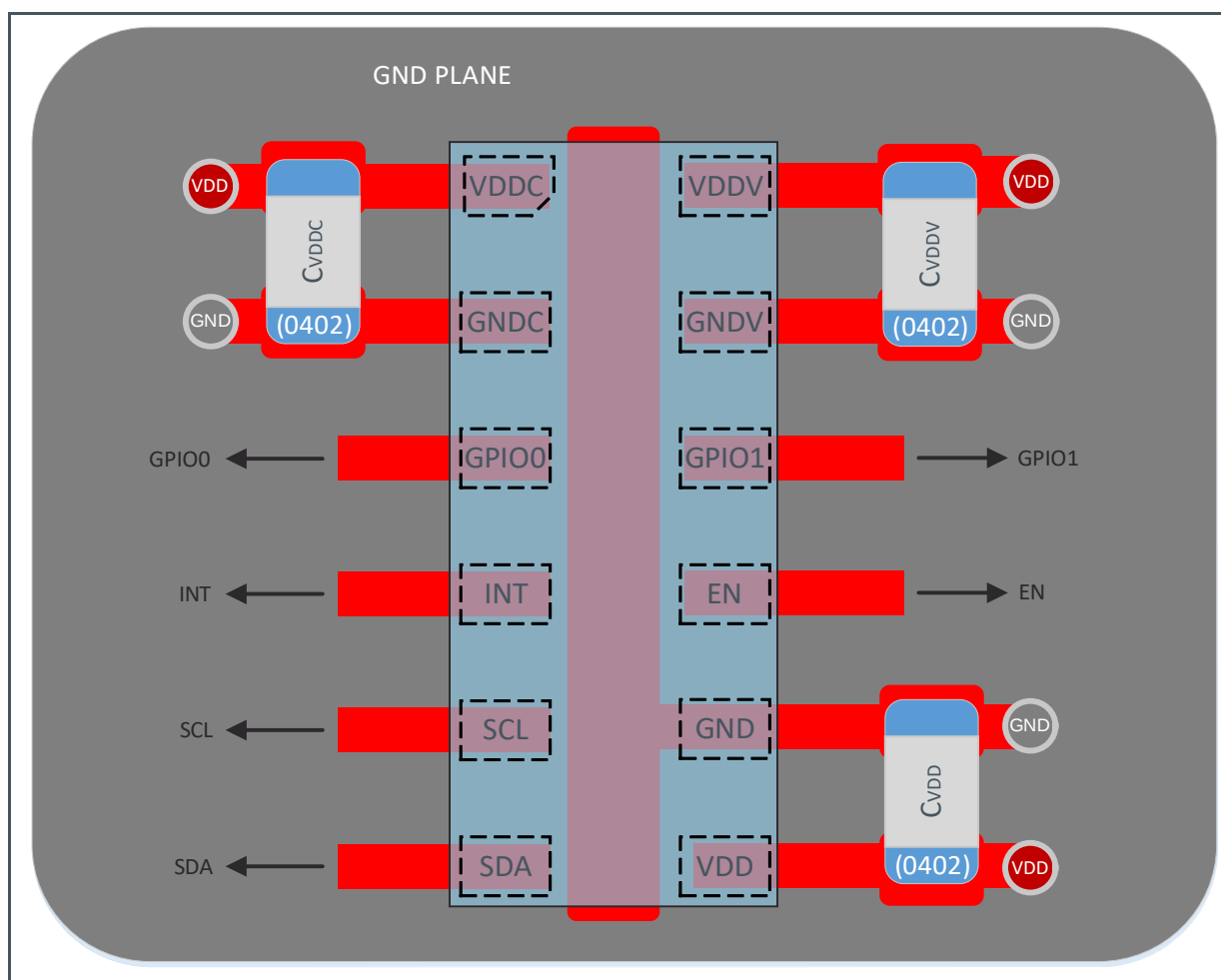
Figure 150: PCB Layout Recommendation
