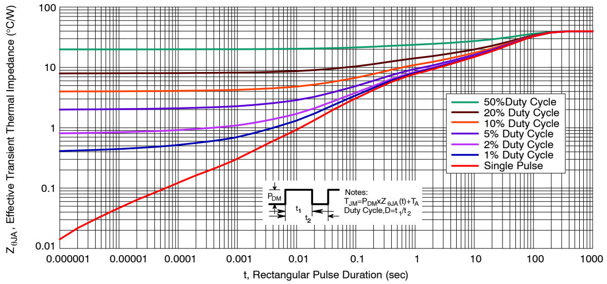
Figure 13. Thermal Characteristics
