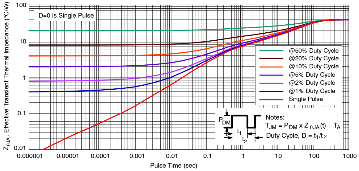
Figure 13. Thermal Response
