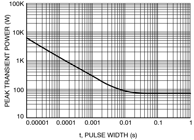
Figure 10. Peak Power
