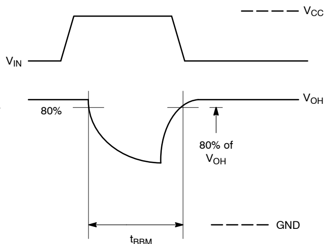
Figure 10. Break-Before-Make Time
