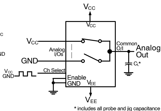
Figure 12. Propagation Delay, Select to Analog Out
