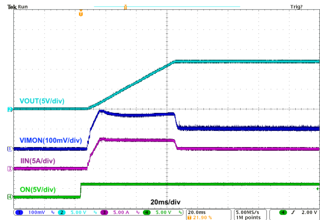
Figure 15. Start-up by ON, I_{OUT} = 5\text{ A} , C_{OUT} = 10\text{ mF}
