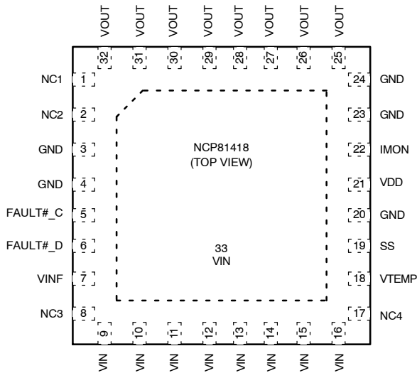
Figure 2. Pin Connections
