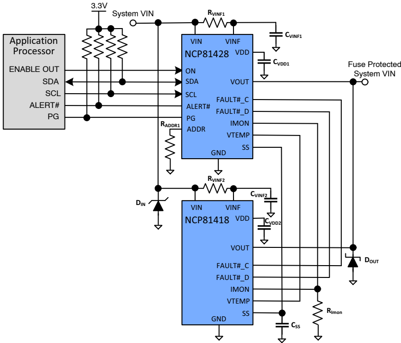
Figure 1. Application Diagram
