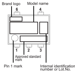
DIP 6-pin Surface-mounting Terminals
