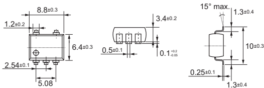
Surface-mounting Terminals
