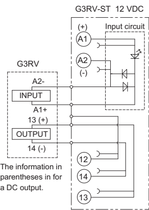
Terminal Arrangement/ Internal Connection Diagram (TOP VIEW)
