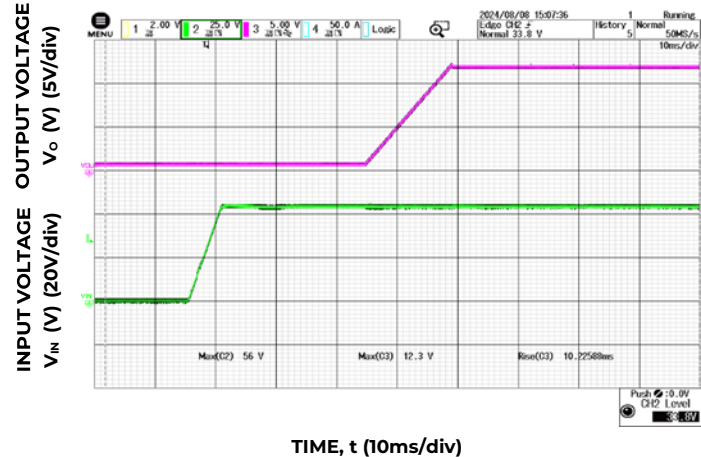
Figure 6. Typical Start-up Using Input Voltage (V IN = 54V, I o = I o,max )
