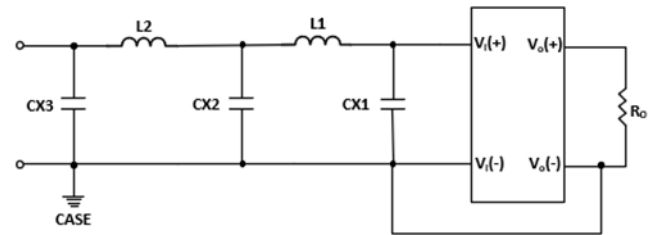
Figure 11. Optional external filter for Class A
