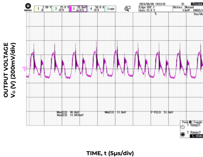
Figure 3. Typical output ripple and noise (C o = 250μF Ceramic + 3900μF PosCap Oscon, V IN = 54V, I o = I o,max )
