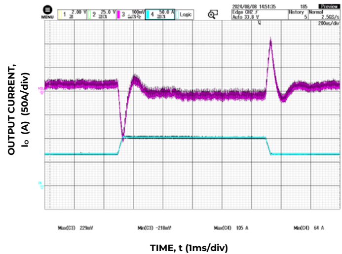
Figure 4. Dynamic Load Response, di o /dt=1A/μs; V IN =V IN,nom ; T A =25°C; Load Change from I o = 50% to 75% of I o,max ; C o = 250μF Ceramic + 3900μF PosCap Oscon
