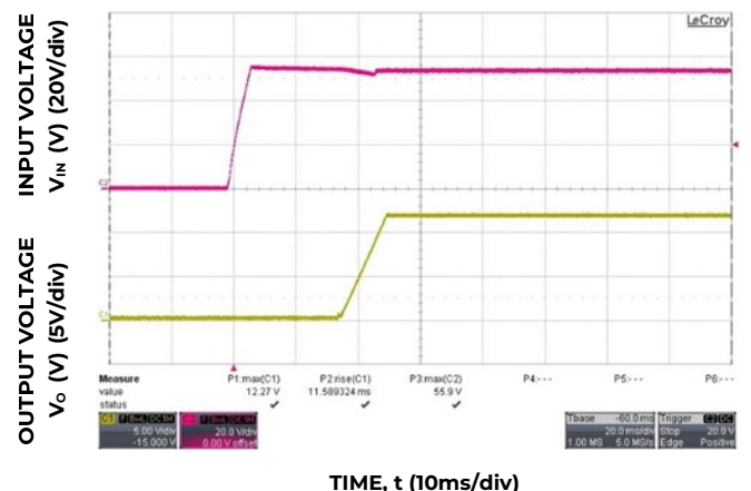
Figure 6. Typical Start-up Using Input Voltage ( V_{in} = 54\text{V} , I_o = 108\text{A} )
