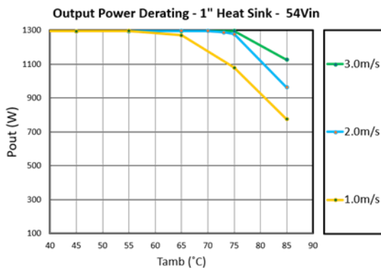
(a) V_{IN}=54V
