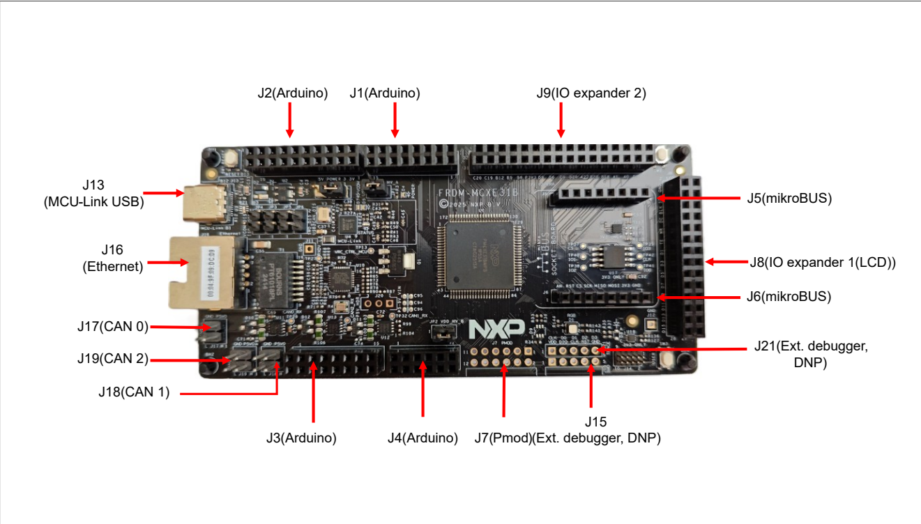
Figure 4. FRDM-MCXE31B board connectors
