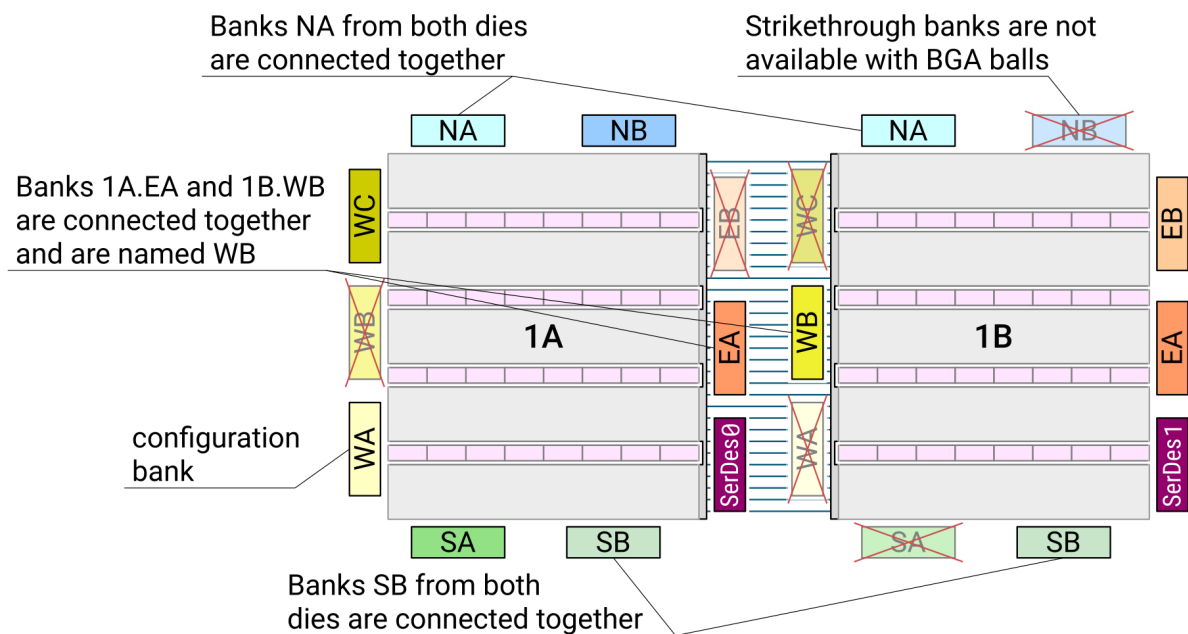
Figure 2.8: GPIO banks of CCGM1A2 (chip view)
