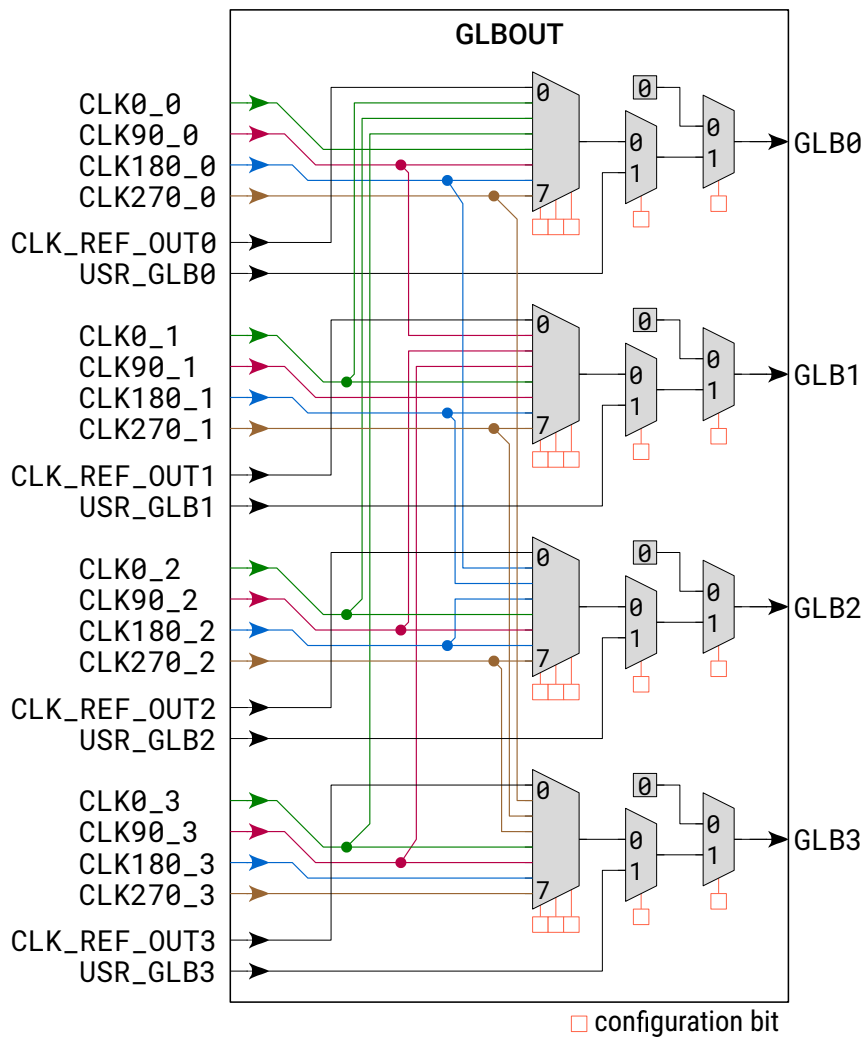
Figure 2.54: GLBOUT multiplexers
