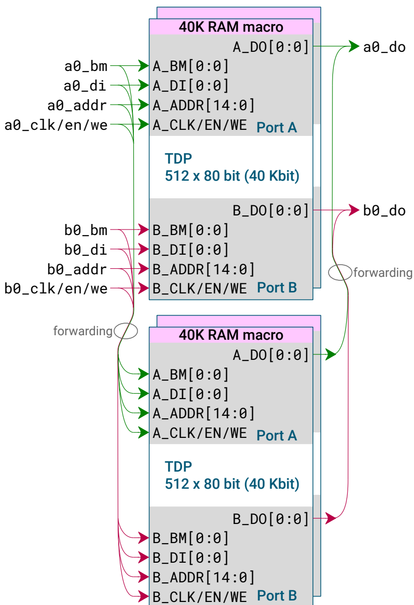
Figure 2.15: Structure of two adjacent DPSRAMs forming one 64K \times 1 bit memory via cascade feature
