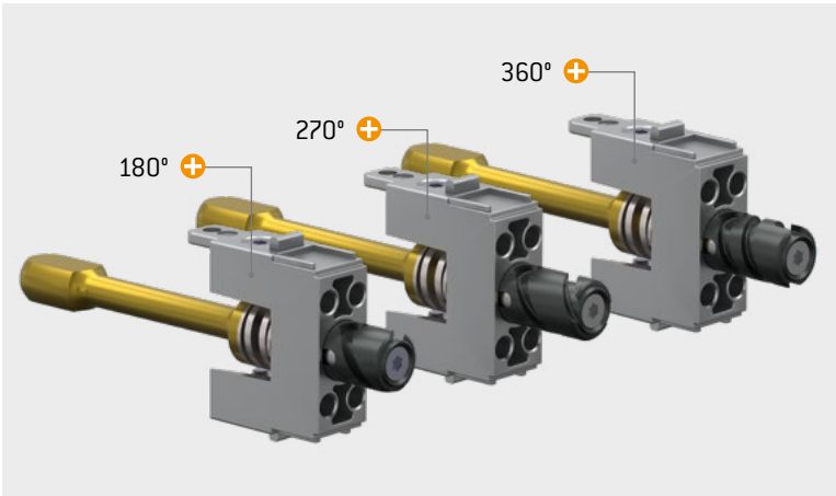
SPINDLE 1 – 12 mm (180°)
