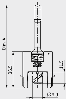
SPINDLE 1 – 11.5 mm (180°)
