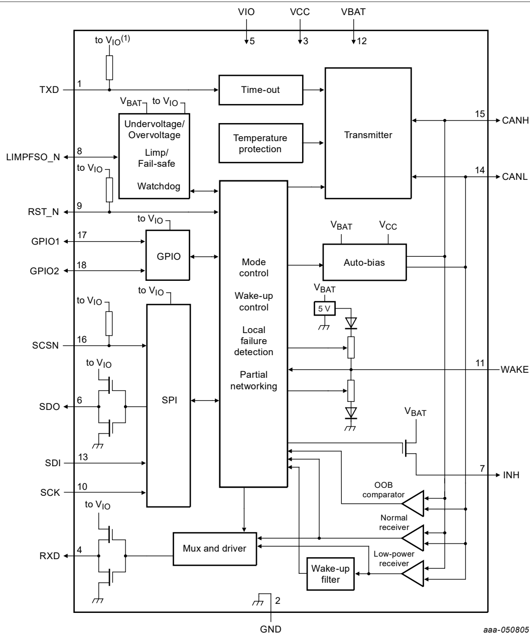
Figure 1. Block diagram
