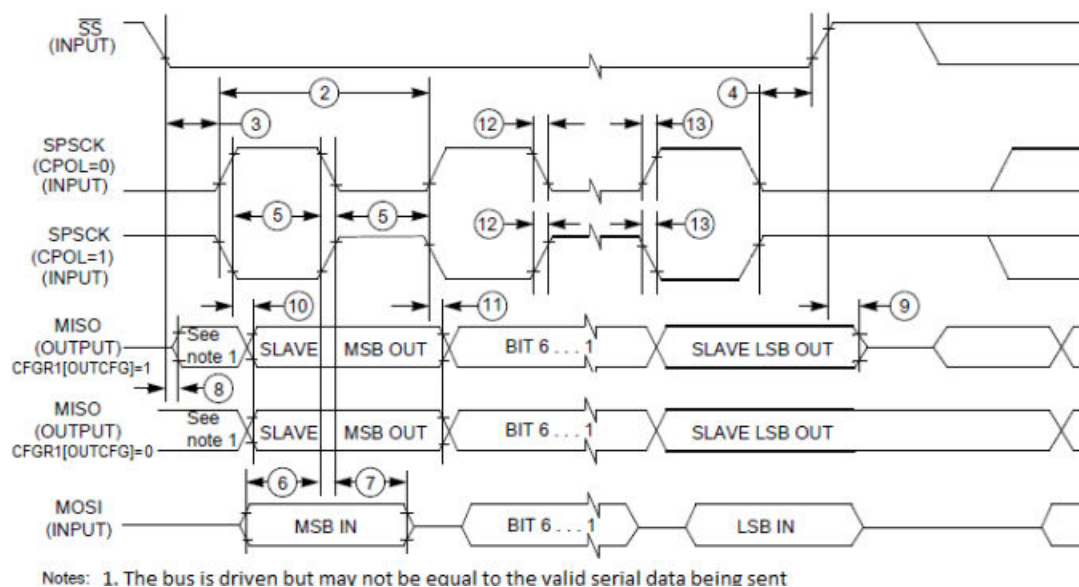
Figure 33. LPSPi slave mode timing (CPHA = 1)
