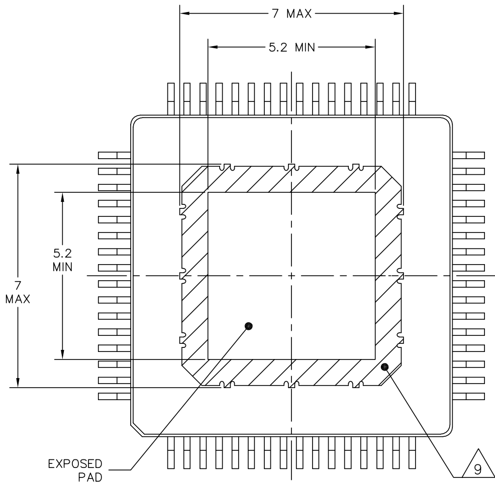
VIEW J—J
