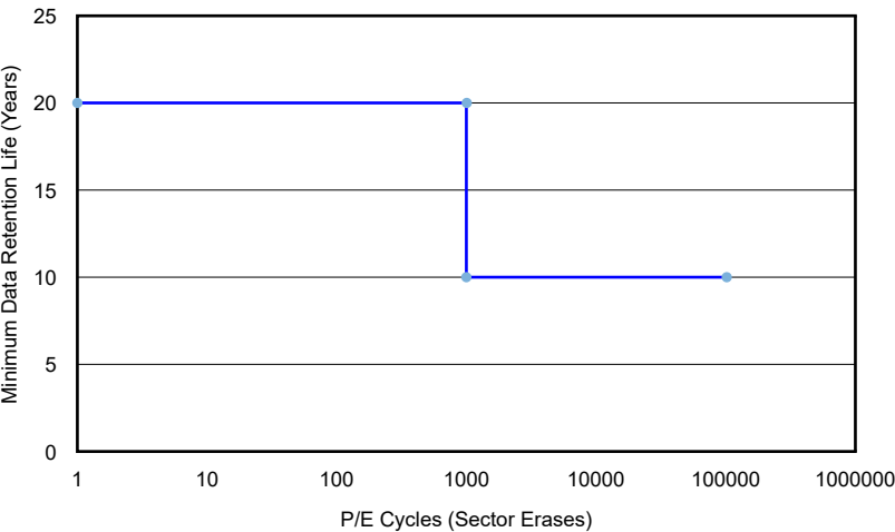
Figure 16. Data retention vs program/erase cycles
