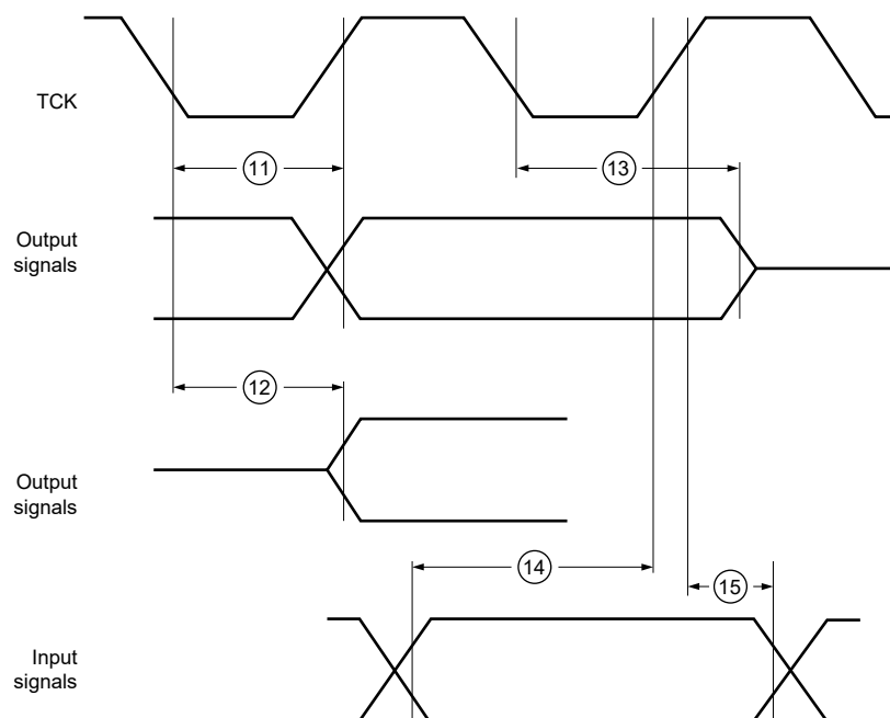
Figure 44. Boundary Scan Timing
