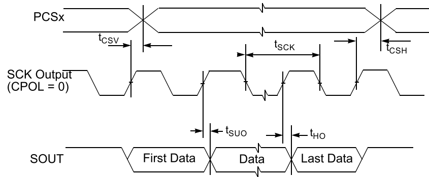
Figure 38. SPI master timing, output only
