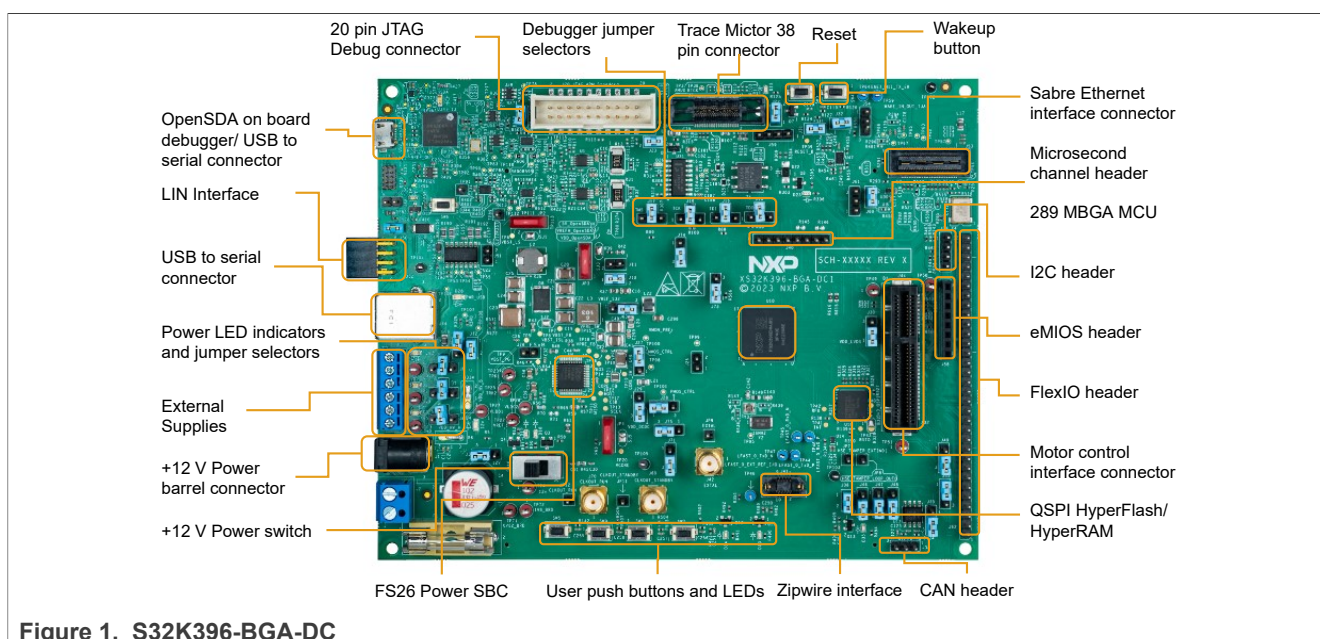
Figure 1. S32K396-BGA-DC
