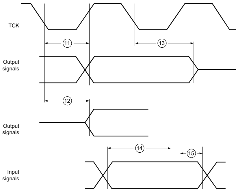
Figure 71. Boundary Scan Timing
