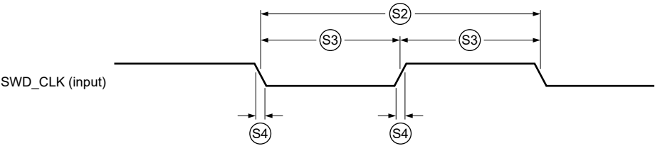
Figure 67. SWD Input Clock Timing
