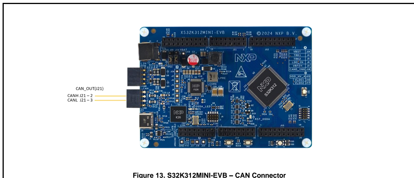
Figure 13. S32K312MINI-EVB – CAN Connector
