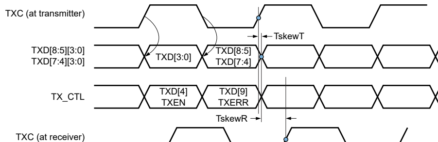
Figure 55. RGMII Transmit Timing
