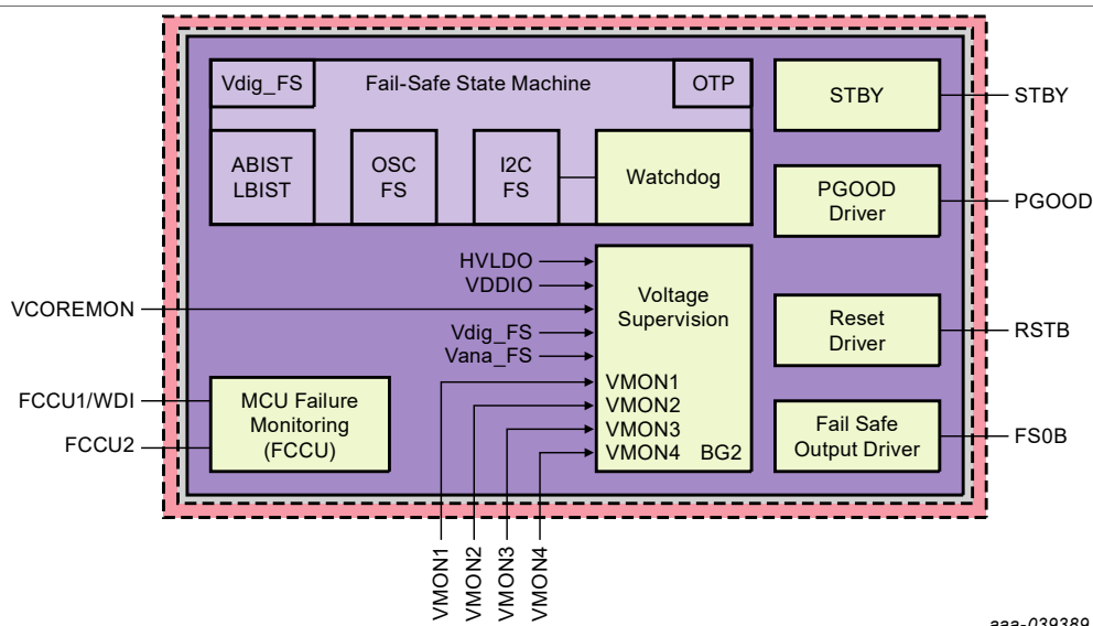
Figure 29. Fail Safe block diagram
