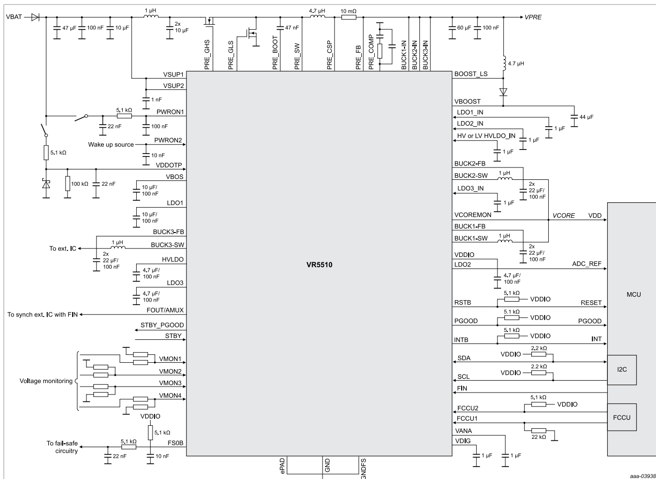
Figure 28. Application schematic
