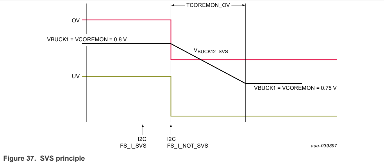
Figure 37. SVS principle
