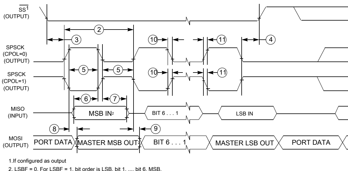
Figure 24. LPSPI master mode timing (CPHA = 1)
