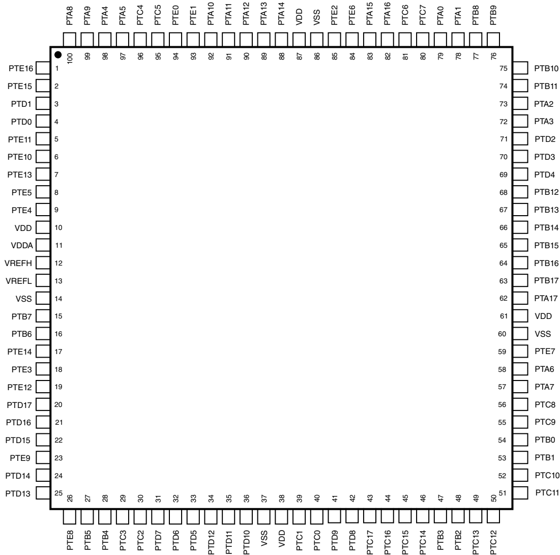
Figure 5. 100 LQFP pinout diagram
