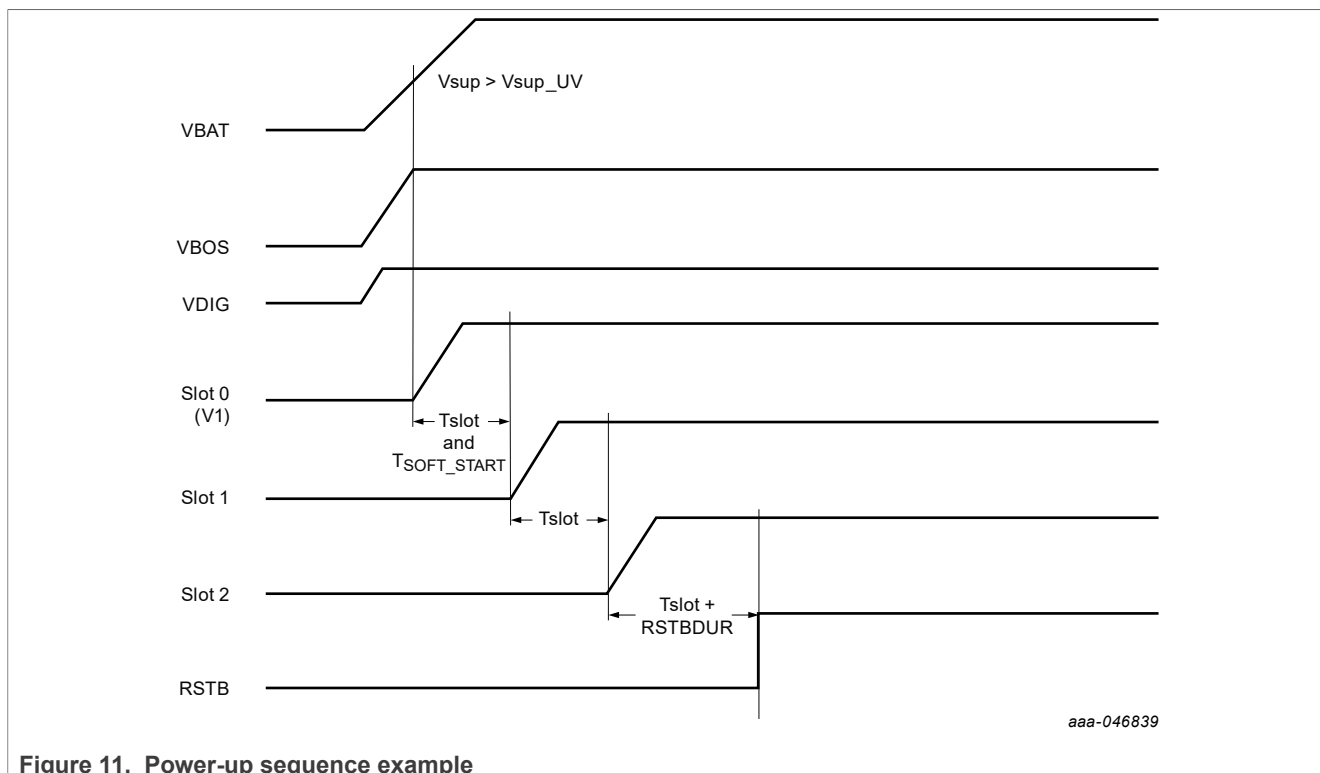
Figure 11. Power-up sequence example
