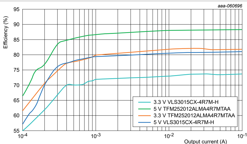
Figure 23. HVBUCK PFM efficiency
