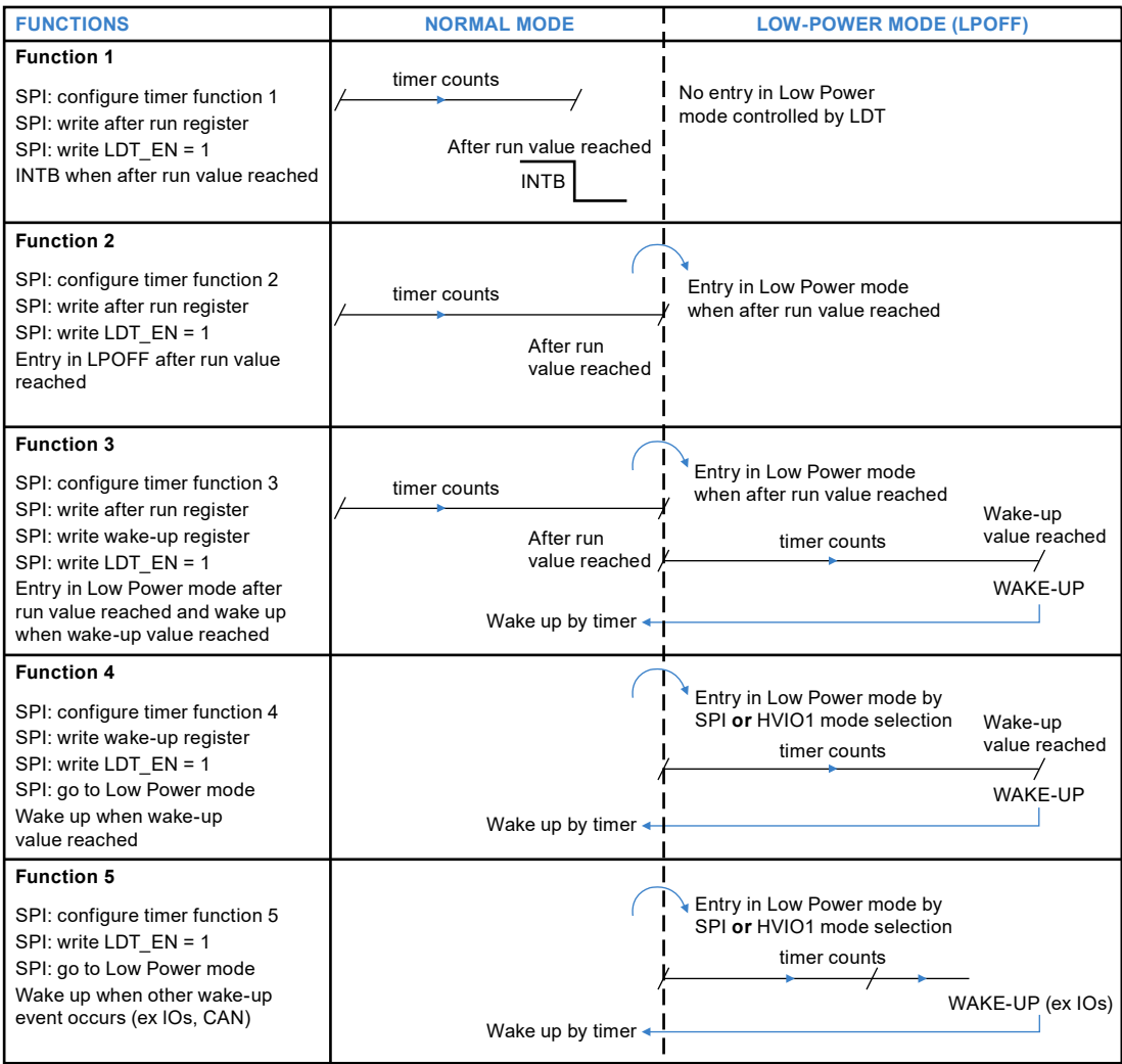
Figure 32. Long duration timer functions
