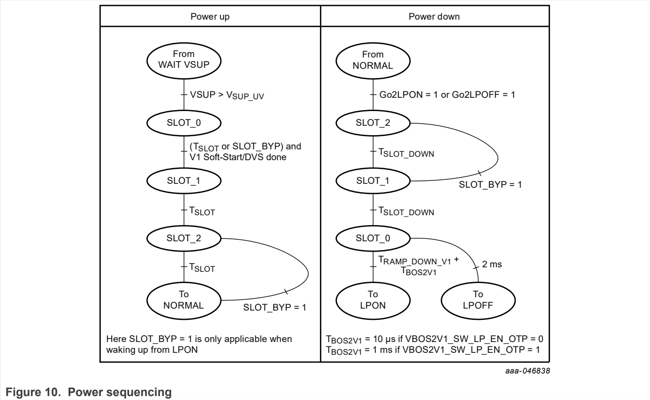
Figure 10. Power sequencing
