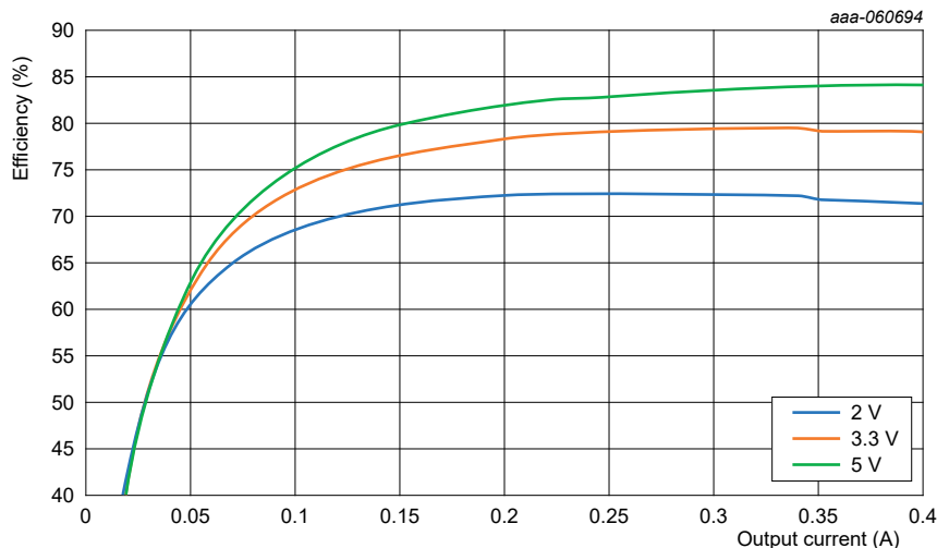
Figure 22. HVBUCK efficiency at 2.25 MHz using VLS3015CX-4R7M-H
