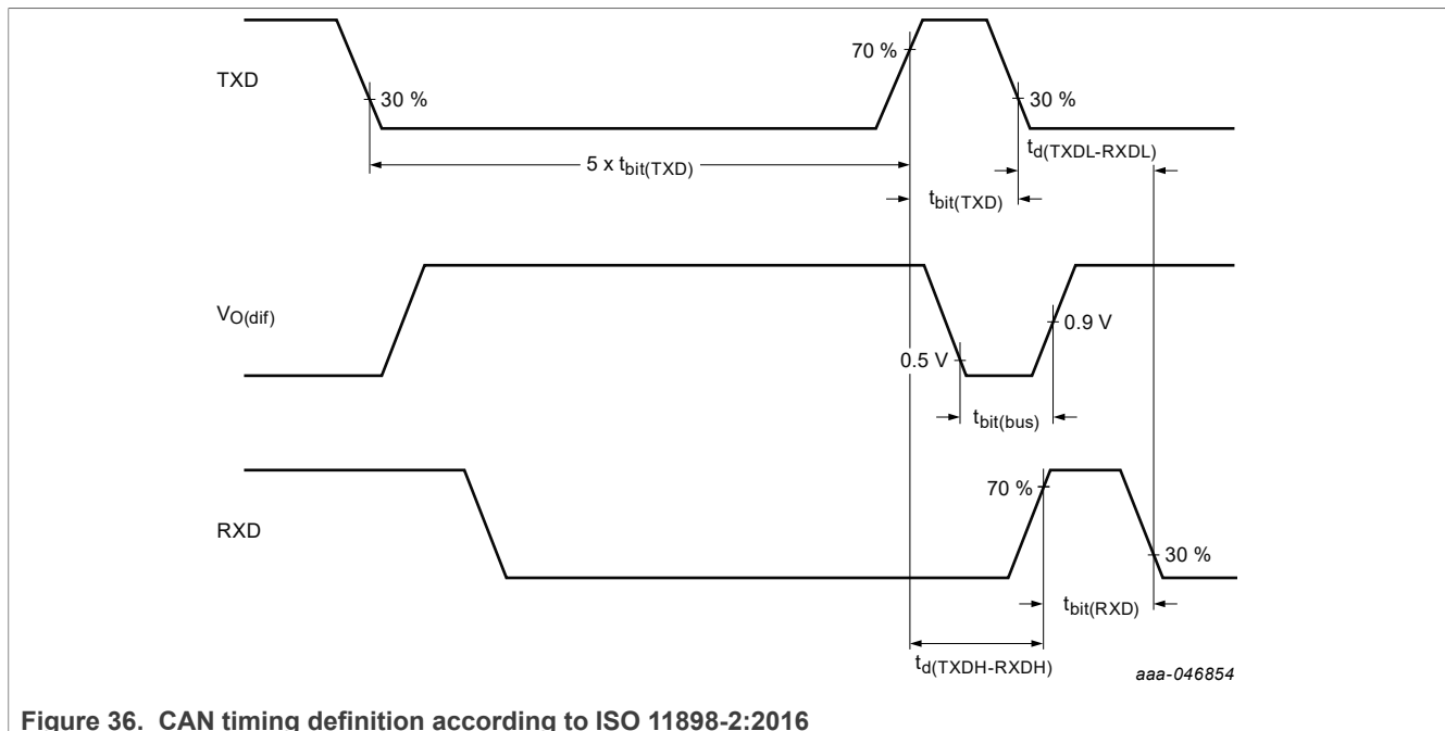
Figure 36. CAN timing definition according to ISO 11898-2:2016
