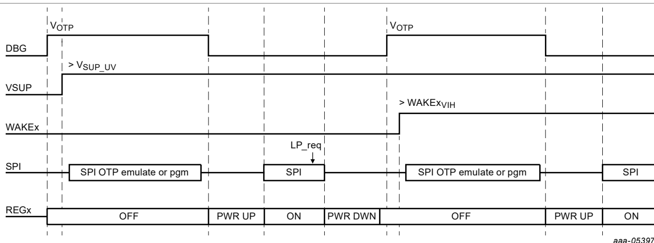
Figure 13. OTP mode time chart
