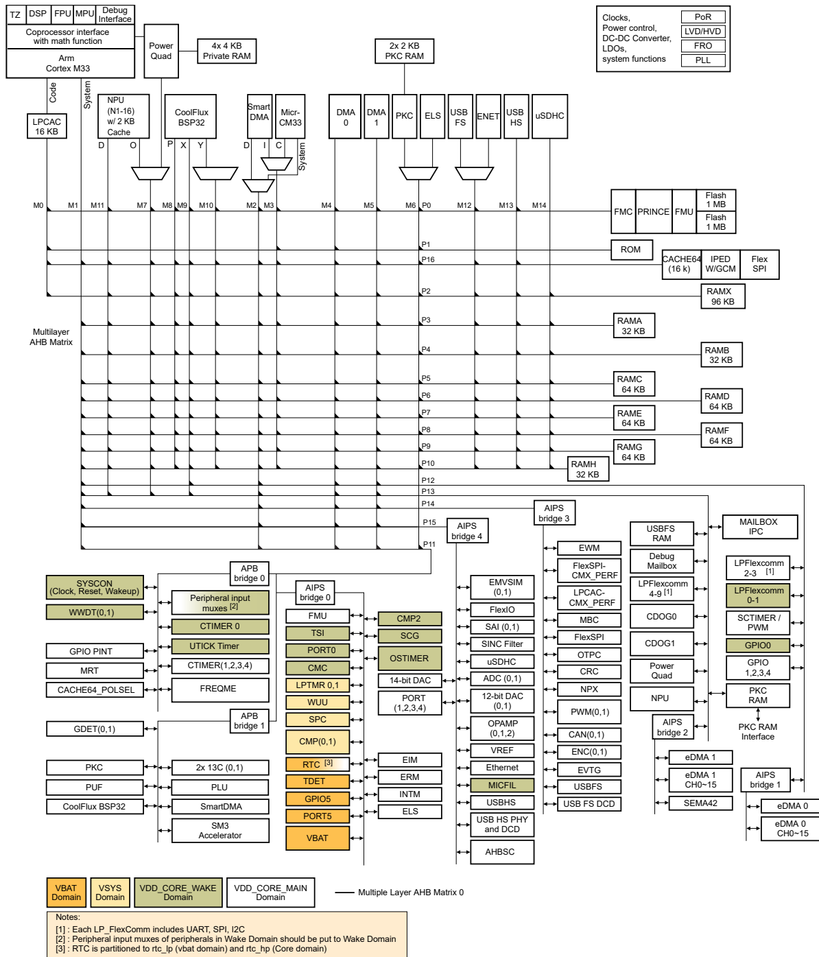
Figure 2. MCX N94x / N54x Architecture
