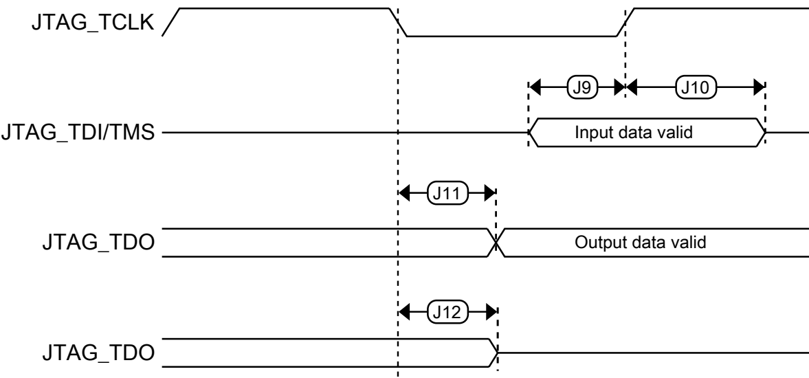
Figure 10. JTAG-DP/TAP timing
