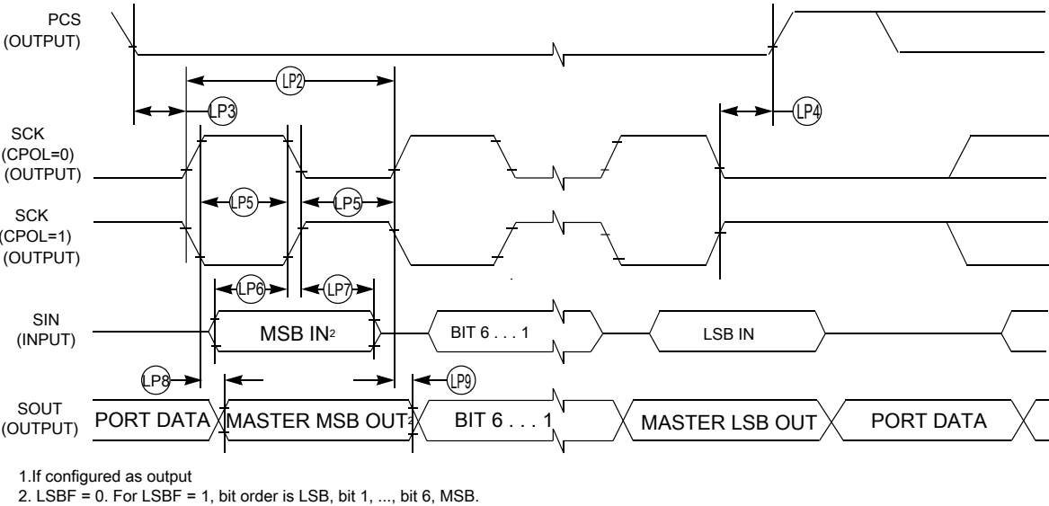
Figure 21. LPSPI master mode timing (CPHA = 1)
