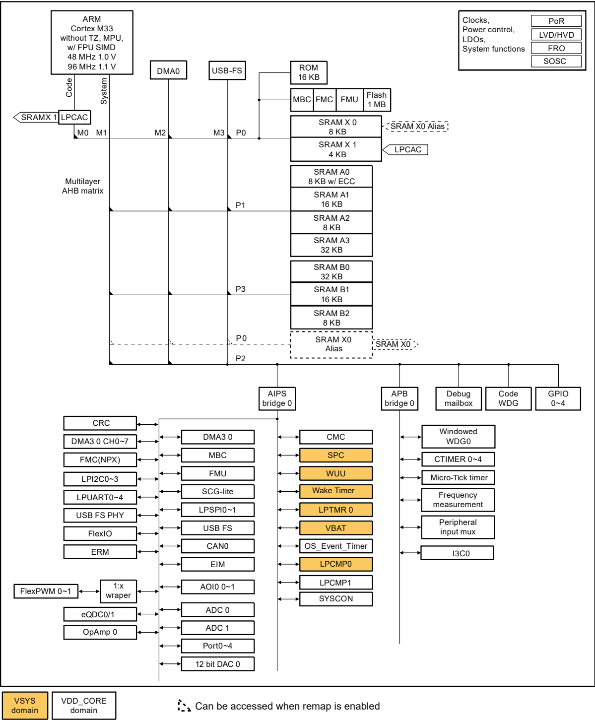
Figure 2. Bus Architecture
