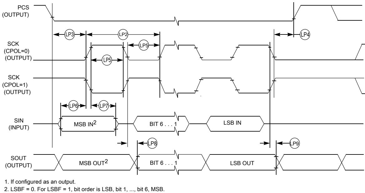
Figure 20. LPSPI master mode timing (CPHA = 0)
