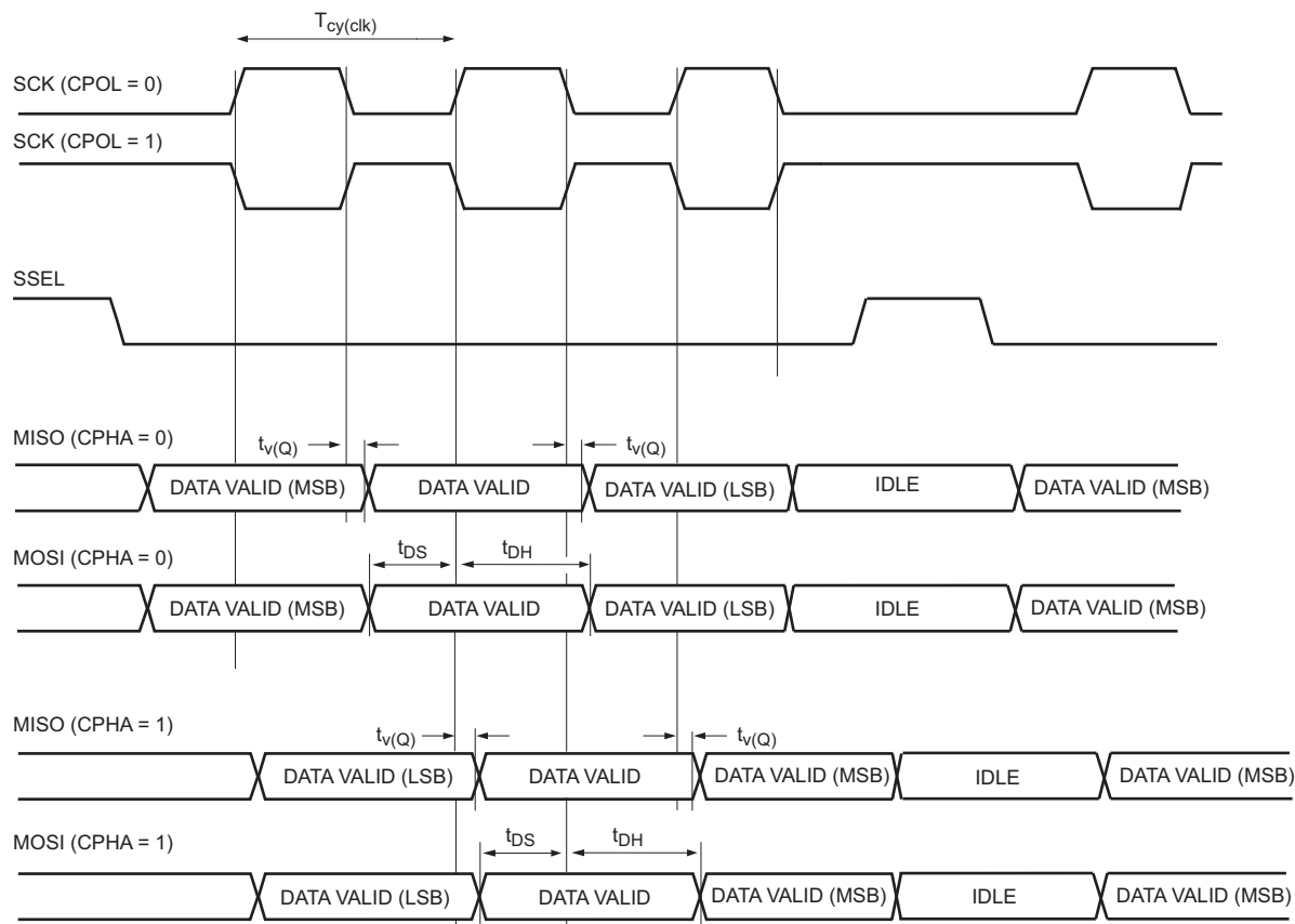
Fig 17. SPI slave timing
