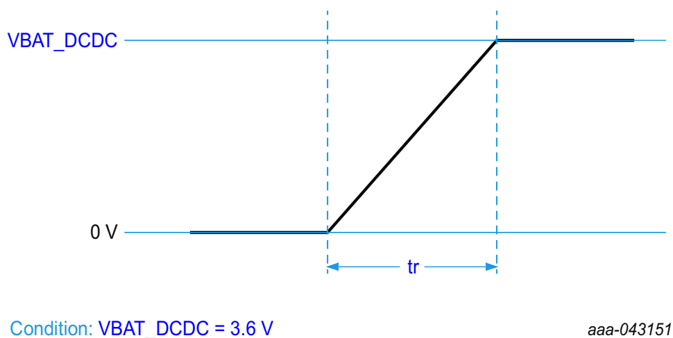
Fig 10. Power-up ramp
