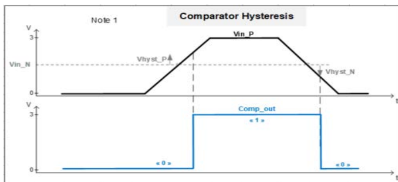
Fig 20. Comparator Hysteresis
