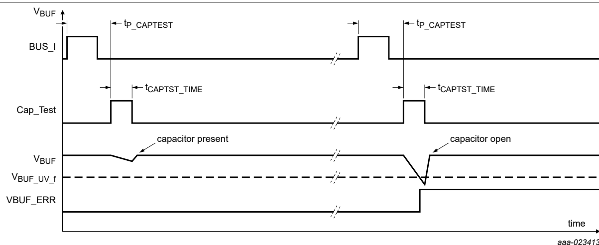
Figure 5. V_{BUF} capacitor monitor timing, PSI5 synchronous mode
