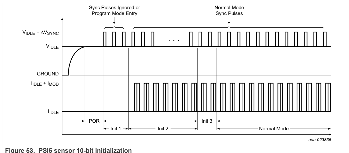
Figure 53. PSI5 sensor 10-bit initialization
