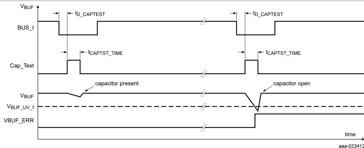
Figure 4. V_{BUF} capacitor monitor timing, DSI3
