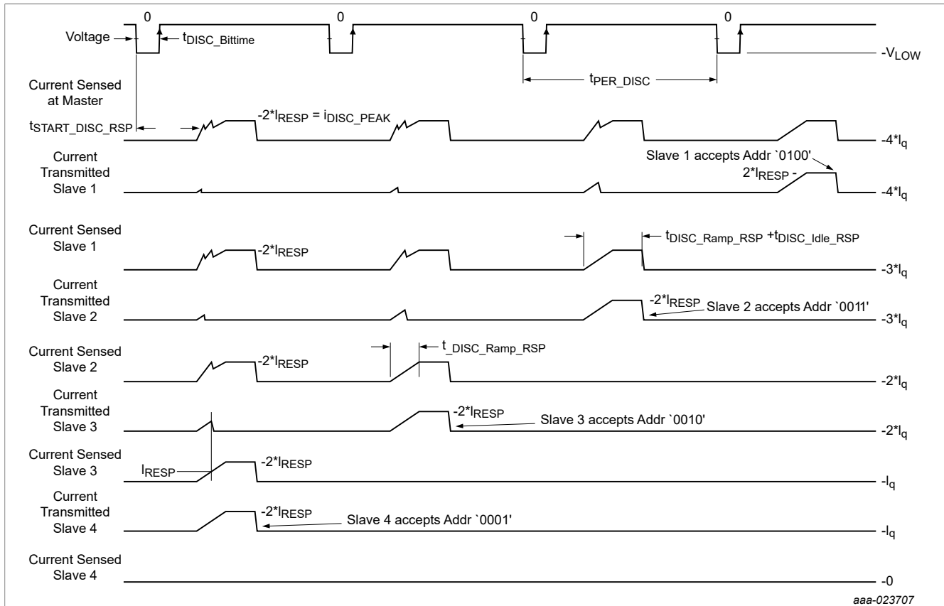
Figure 33. DSI3 discovery mode timing diagram
