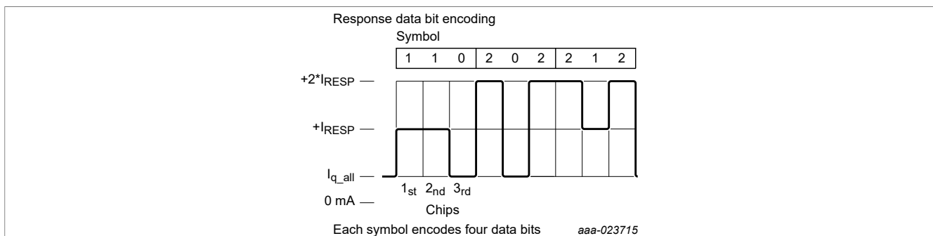
Figure 37. Response symbol encoding
