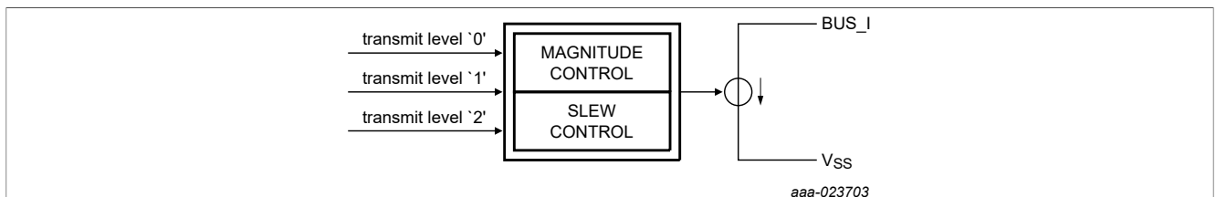
Figure 30. DSI3 transmitter block diagram
