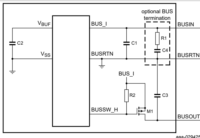
Figure 59. DSI3 switch connected daisy chain application diagram
