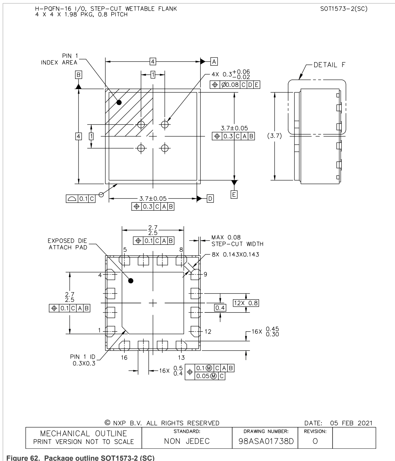
Figure 62. Package outline SOT1573-2 (SC)
