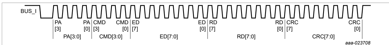
Figure 34. Command and response mode command example
