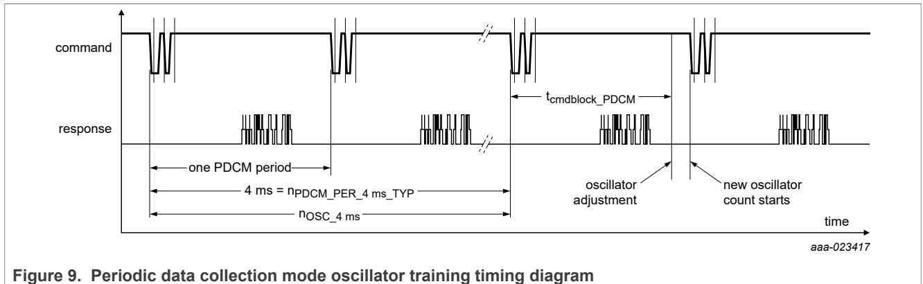
Figure 9. Periodic data collection mode oscillator training timing diagram
