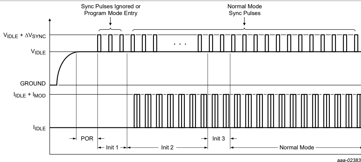
Figure 30. PSl5 sensor 10-bit initialization
