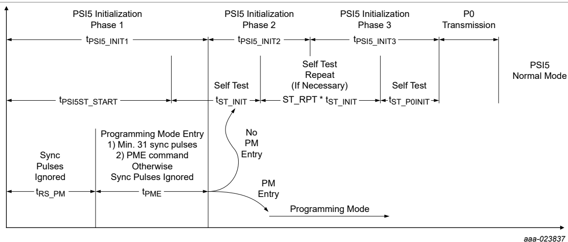
Figure 31. PSI5 initialization timing, synchronous mode
