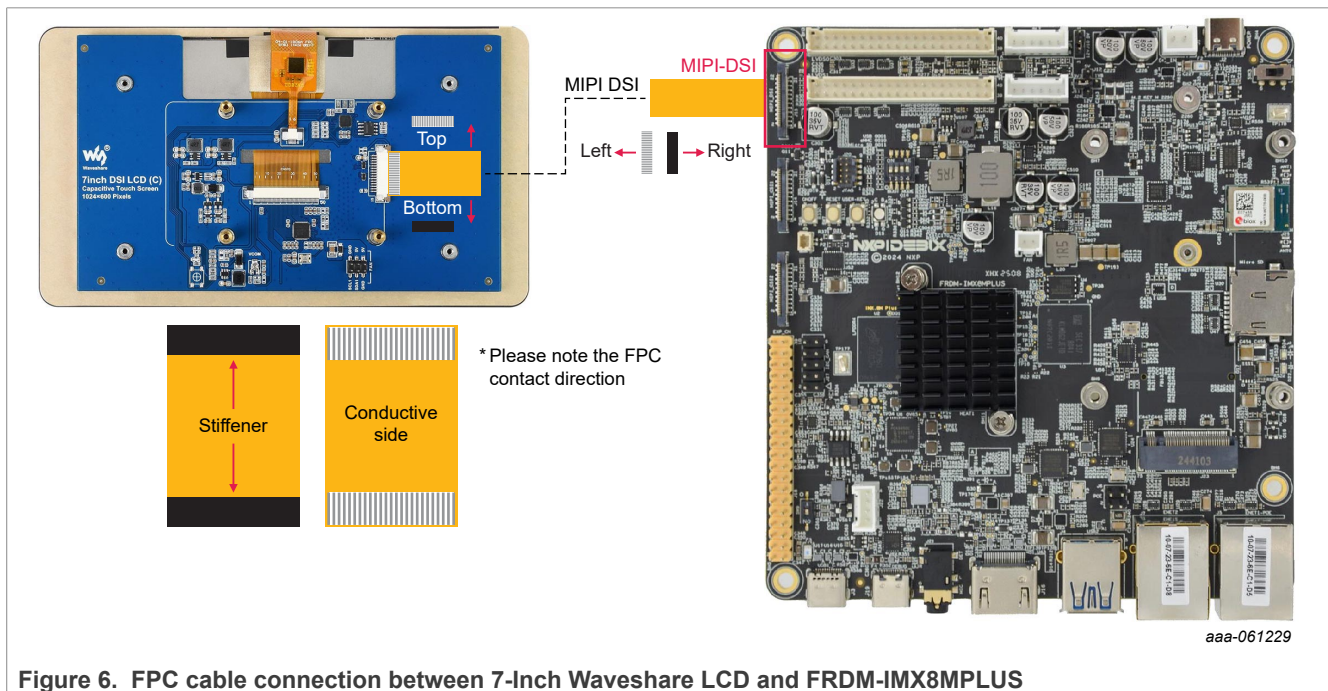
Figure 6. FPC cable connection between 7-Inch Waveshare LCD and FRDM-IMX8MPLUS
