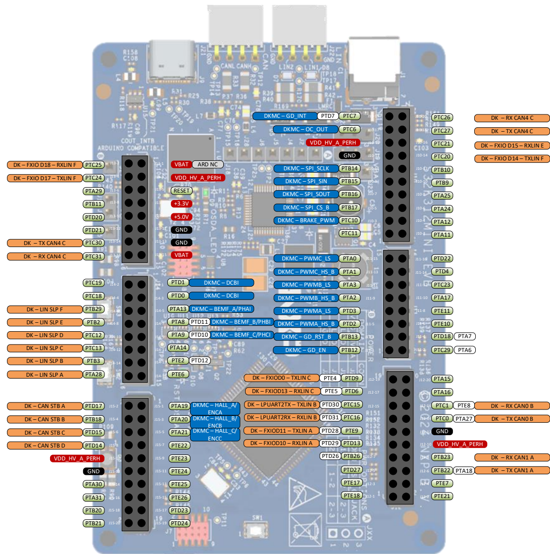
Figure 18. S32K312MINI-EVB - DEVKIT MOTORGD/COMM
