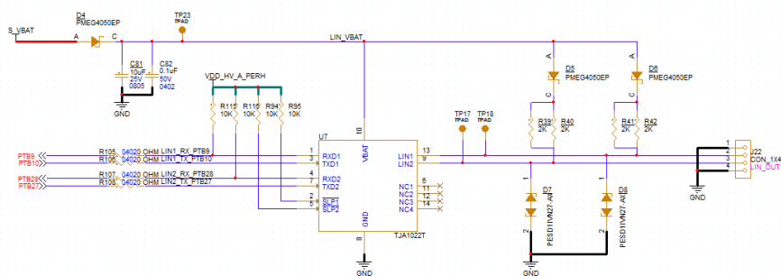
Figure 12. S32K312MINI-EVB - LIN Interface Connection
