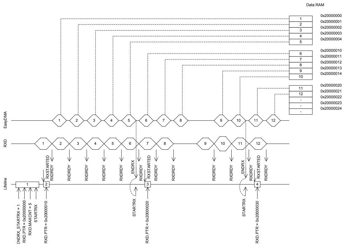
Figure 97: UARTE reception
