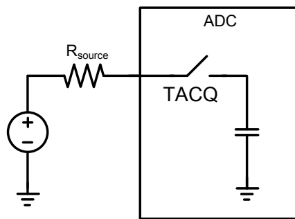
Figure 105: Simplified ADC sample network
