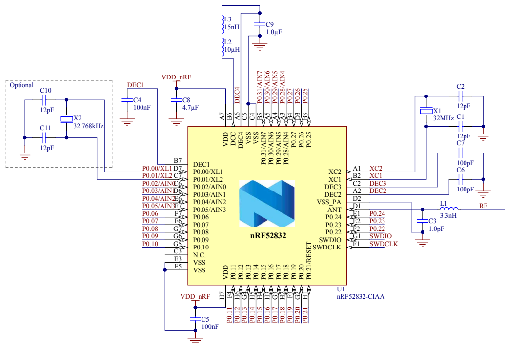
Figure 175: CIAA WLCSP with DC/DC regulator setup
