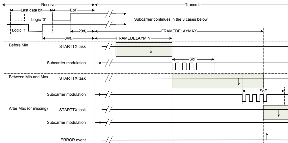
Figure 121: Frame timing controller (FRAMEDELAYMODE=Window)
