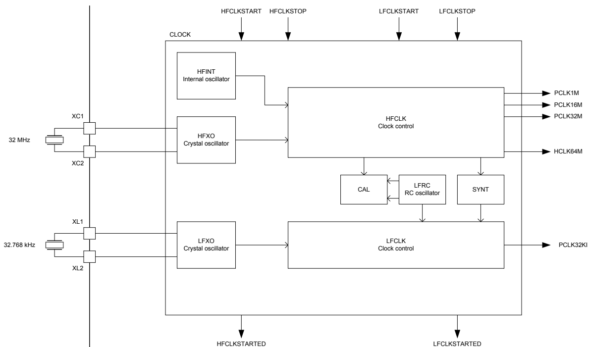
Figure 19: Clock control
