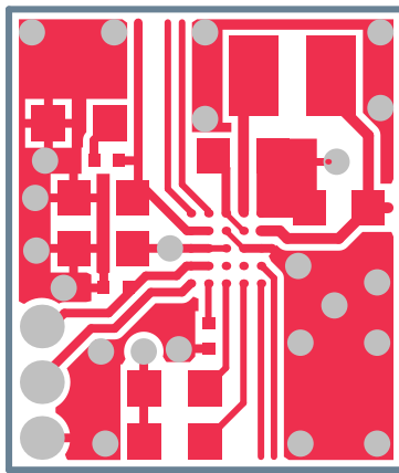
Figure 38: Top layer
