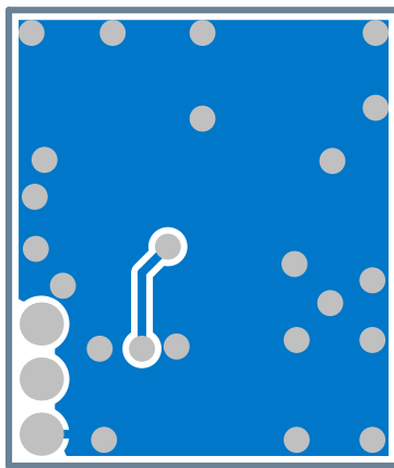
Figure 39: Bottom layer
