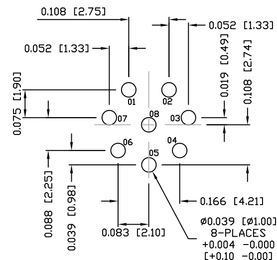
PCB LAYOUT
