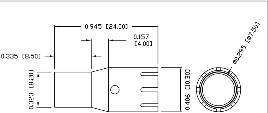
BACK SHELL OPTION "O"
