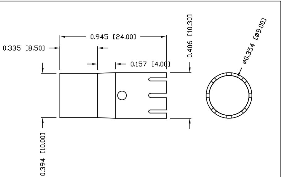
RECOMMENDED CRIMPING INSTRUCTIONS OPTION "L"
